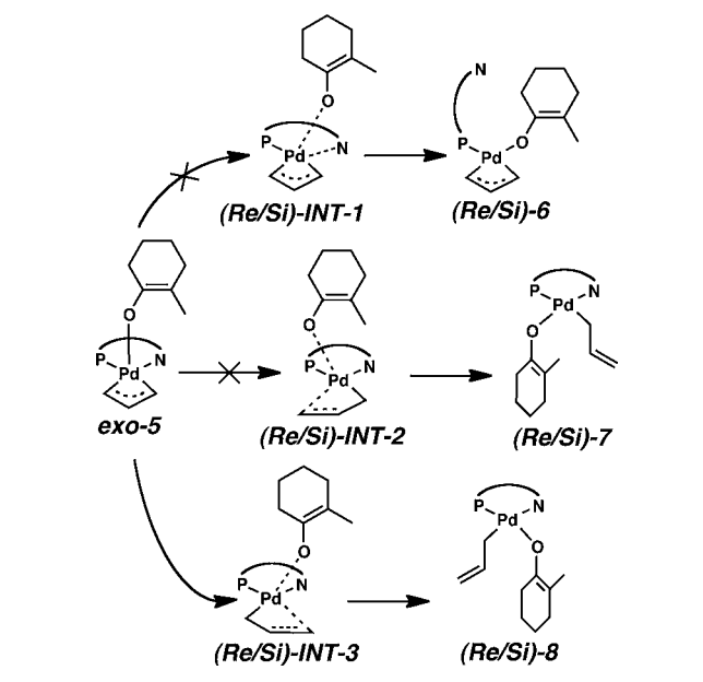
Scheme 4. Internal Rearrangement Mechanisms Considered in This Work
