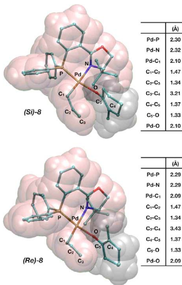
Figure 8. Representations of 4-coordinate ( Si )-8 and ( Re )-8 (Pd 2+ complexes), formed after inner-sphere ligand rearrangement. The table displays relevant interatomic distances.
