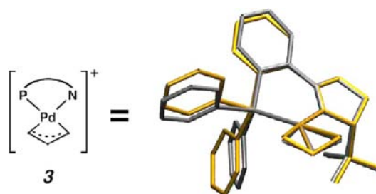
Figure 1. Superimposed calculated (yellow) and experimentally obtained solid-state (silver) structure for \pi -allyl complex 3 . The experimental crystal structure was obtained using \text{PF}_6^- as the counterion.
